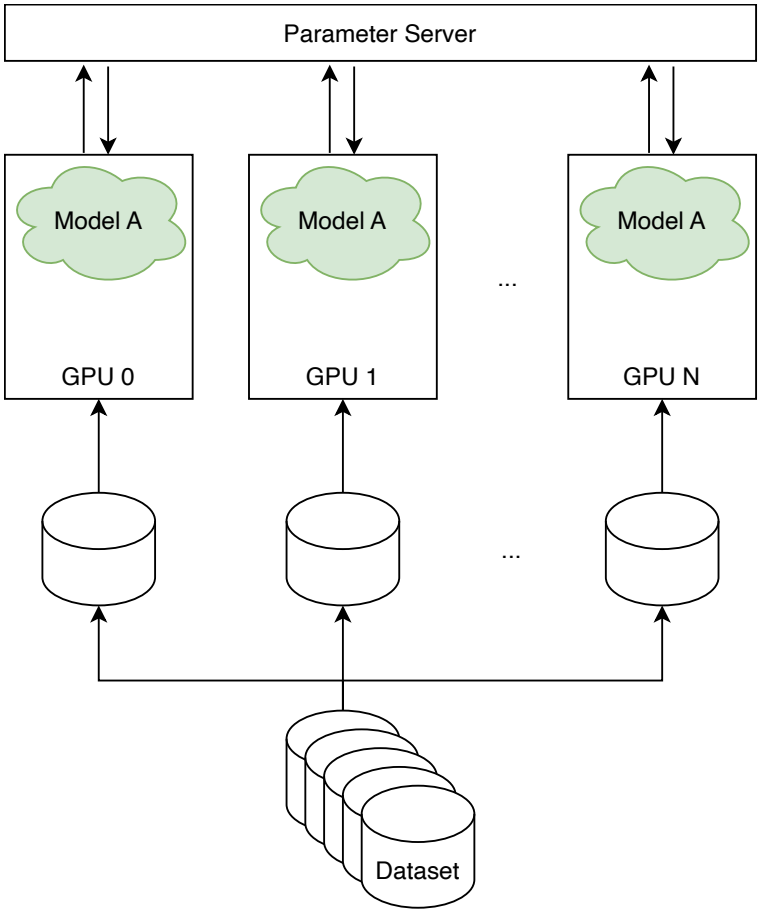
Figure 21: Data parallelism
