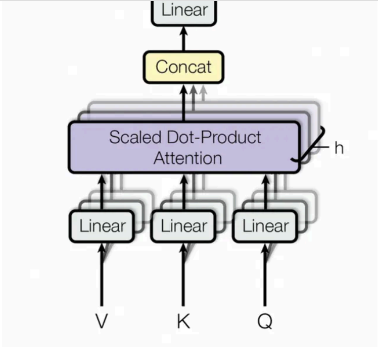
Figure 18: Multi-head attention (Credit: [32])
