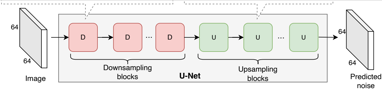
Figure 16: U-Net architecture
